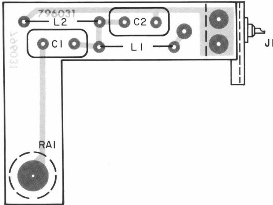
Figure 1-4. Type 796031 Matching Network Assembly (A2), Location of Components
